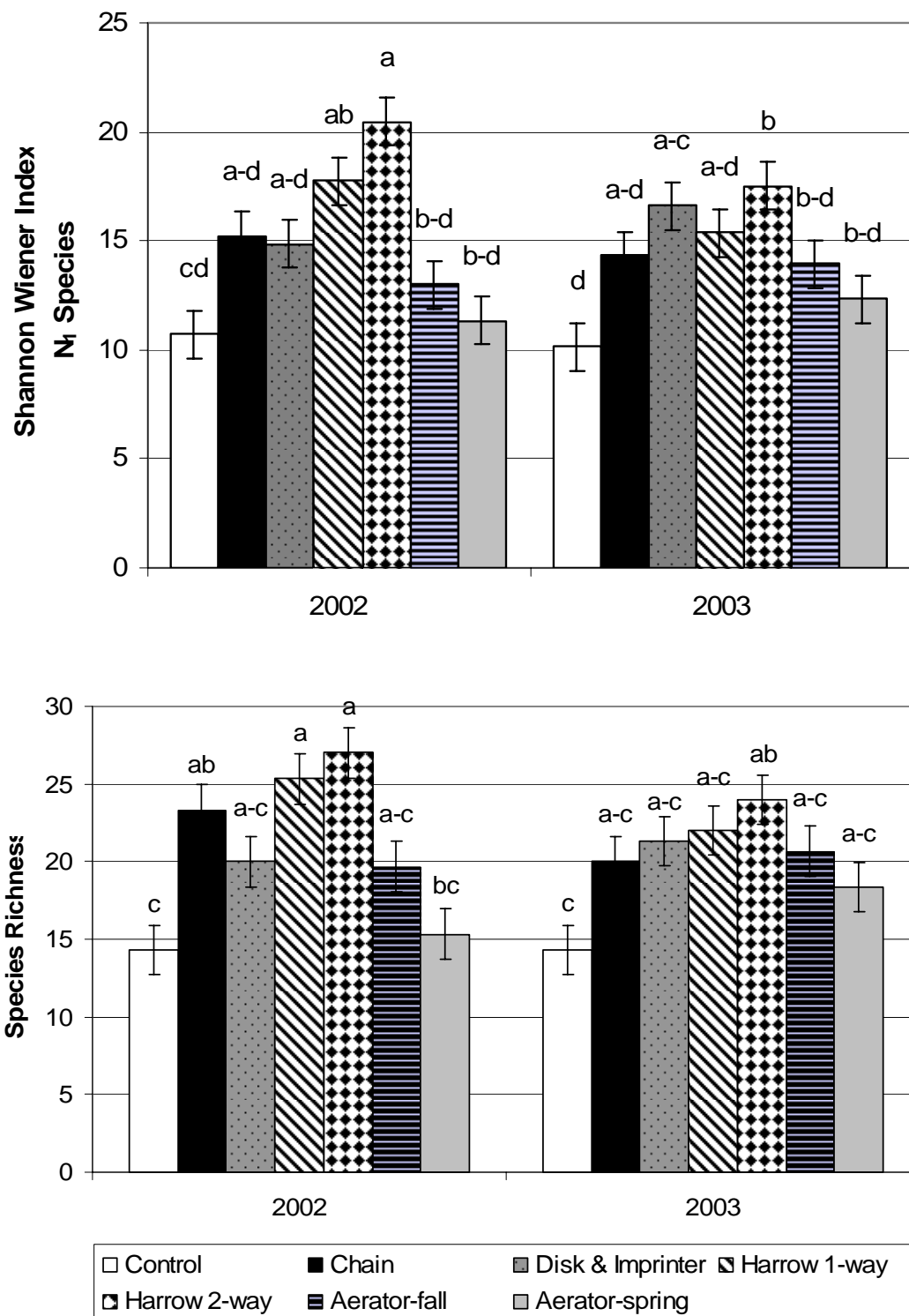
Fig. 1. Shannon Wiener index (above) of species diversity, where N_i (\pm SE) is equal to the number of equally common species. Mean ( \pm SE ) species richness (below) for each treatment. Different letters indicate a significant difference within and across years ( P < 0.05 ).
